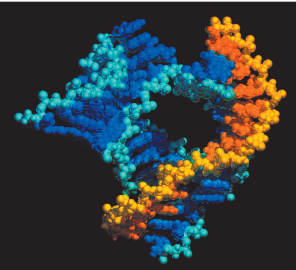
Molecular image of the hammerhead ribozyme (in blue) bound to RNA (in orange). Ribozymes are catalytic RNA molecules that may have been the first carriers of genetic information. [Kenneth Eward/Photo Researchers.]
