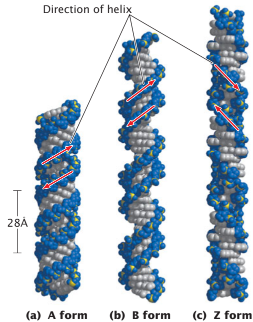
8.13 DNA can assume several different secondary structures.
