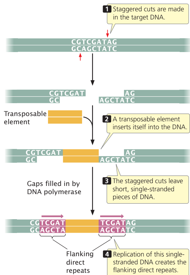
13.23 Flanking direct repeats are generated when a transposable element inserts into DNA.
