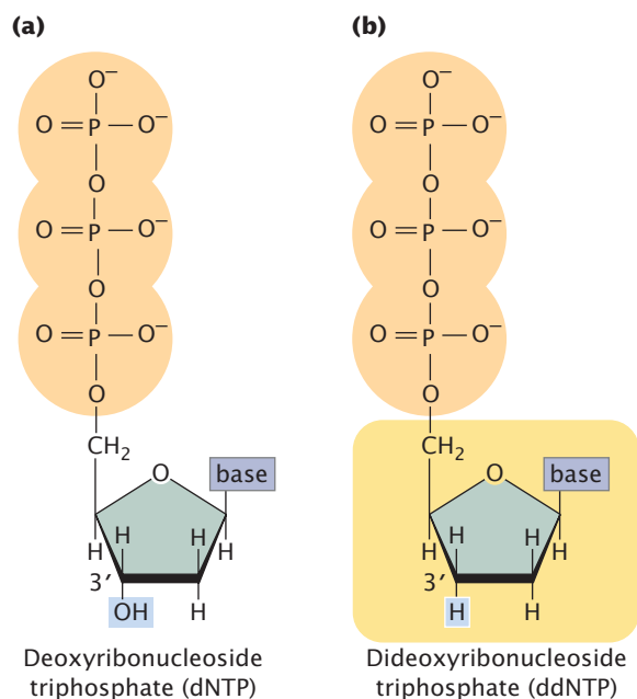
14.13 The dideoxy sequencing reaction requires a special substrate for DNA synthesis. (a) Structure of deoxyribonucleoside triphosphate, the normal substrate for DNA synthesis. (b) Structure of dideoxyribonucleoside triphosphate, which lacks an OH group on the 3'-carbon atom.
